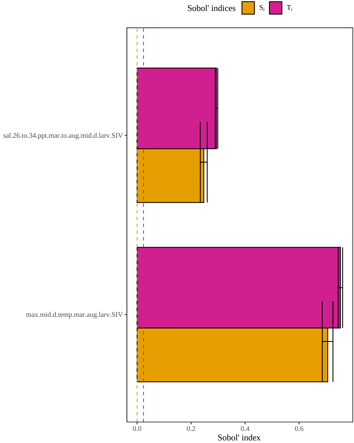
Figure 3. Results of a sensitivity analysis for the redkingcrabLarv model based on the original weighted geometric mean model outlined in Jewett and Onuf (1988). Dashed lines represent baseline numerical approximation error for S_i and T_i ( i.e. , dummy variables).
